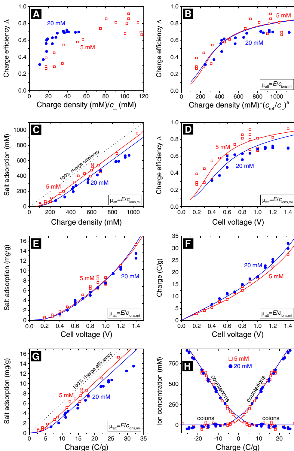
Fig. 3 Analysis of data of salt adsorption and charge efficiency \Lambda for NaCl solutions at c_\infty=5 and 20 mM for cell voltages up to V_{\text{cell}}=1.4 V. a Plotting \Lambda vs. the ratio \sigma_{\text{mi}}/c_\infty does not lead to overlap of the datasets, demonstrating that using \mu_{\text{att}}=\text{constant} in the standard mD model is not correct. b Plotting \Lambda vs. \sigma_{\text{mi}} \cdot (c_{\text{ref}}/c_\infty)^a with a=0.31 leads to a perfect overlap of the modeling lines, where \mu_{\text{att}}=E/c_{\text{ions,mi}} and E=300 kT mol/m 3 . The datasets now also overlap quite closely demonstrating the relevance of the use of the improved mD model ( c_{\text{ref}}=20 mM). c Using the improved mD model, the total excess micropore ion adsorption, c_{\text{ions,mi}} (equal to salt adsorption in a symmetric cell pair), is plotted vs. the micropore charge density, \sigma_{\text{mi}} , showing the expected deviation from the 100 % charge efficiency line. d Theory of \Lambda vs. V_{\text{cell}} according to the improved mD model (compared with data), showing a much smaller influence of c_\infty on \Lambda than in the standard mD model; see Fig. 2b in ref. [38]. e–g Direct data of salt adsorption \Gamma_{\text{salt}} in milligrams per gram and charge \Sigma_F in coulombs per gram, compared with the improved mD model. h Calculated micropore ion concentrations as a function of electrode charge, again compared with the improved mD model
