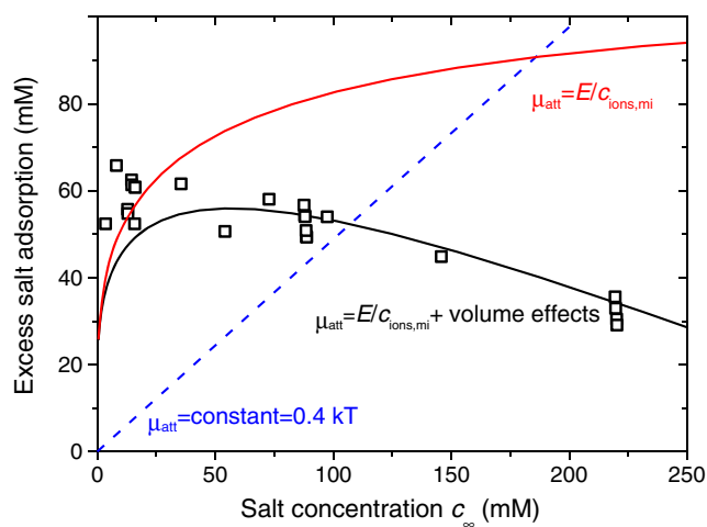
Fig. 6 Excess adsorption of NaCl in uncharged carbon as function of external salt concentration, c_{\infty} . Straight dashed line based on standard mD model (constant \mu_{att} = 0.4 kT), upper curved line based on the improved mD model, and lower curved line for extended model including ion volume effects
