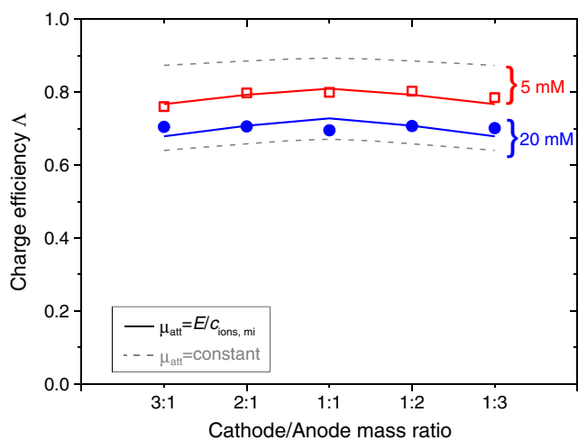
Fig. 5 Charge efficiency for CDI at unequal mass ratio cathode to anode ( V_{cell} = 1.0 V). Dashed lines show prediction using a fixed \mu_{att} in the standard mD model, while the solid lines show results for the improved mD model where \mu_{att} = E/c_{ions,mi}
