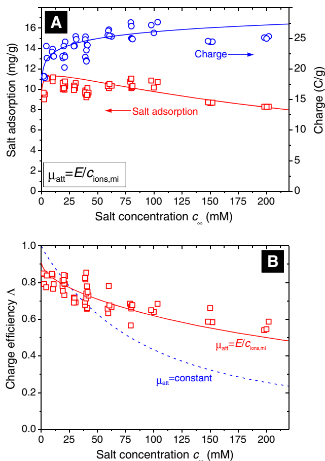
Fig. 4 a Salt adsorption and charge density, and b charge efficiency \Lambda , for CDI in a range of NaCl salt concentrations (2.5–200 mM) at V_{cell} = 1.2 V. Both in a and b , solid lines denote calculation results of the improved mD model, while in b , the dashed line is based on the standard mD model
