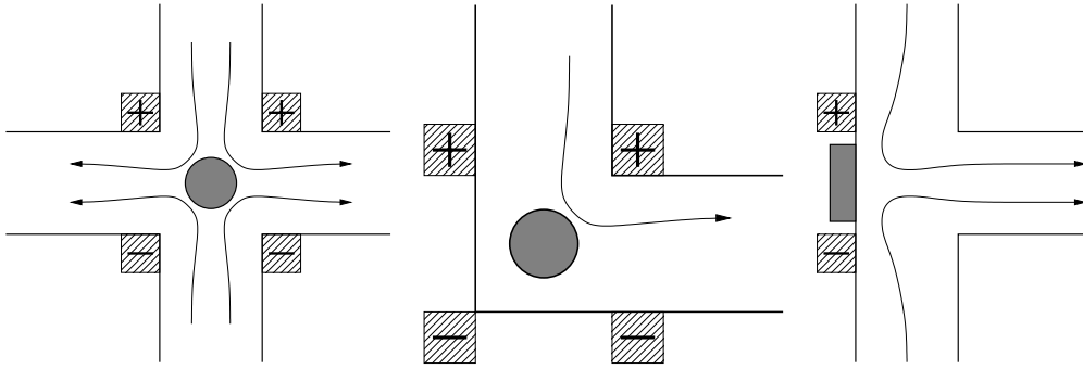
FIGURE 5. ICEO micropump designs for ‘cross-’, ‘elbow-’, and ‘T-’ junctions. A conducting cylinder placed in a junction of microchannels, subject to an applied AC or DC field, drives an ICEO flow which draws fluid in along the field axis and expels it perpendicular to the field axis. For the four-electrode configurations, the field axis can be switched from vertical to horizontal by switching the polarities of two diagonally opposite electrodes, reversing the pumping direction.
